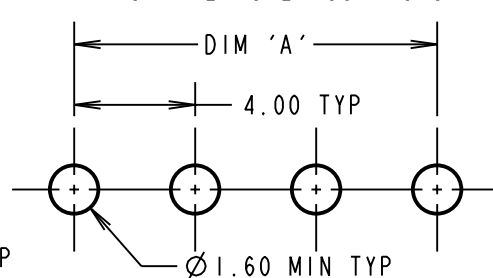
RECOMMENDED PCB LAYOUT FOR ALL PC TAIL POWER CONTACTS
