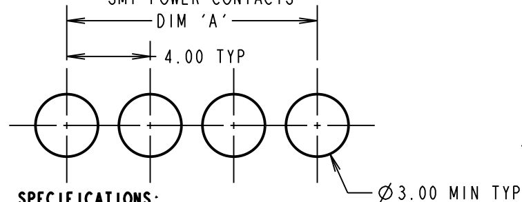
RECOMMENDED PCB LAYOUT FOR ALL SMT POWER CONTACTS
