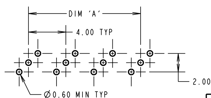
RECOMMENDED PCB LAYOUTS FOR COAX CONTACTS: M80-311/312
