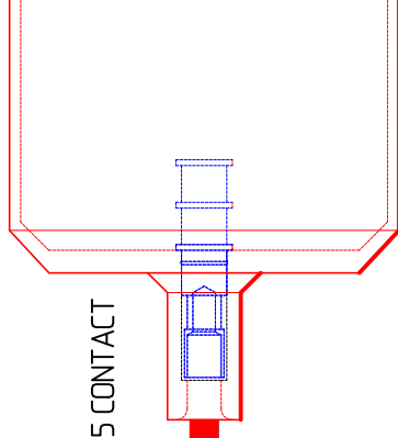
113422R CASING MOULDING
