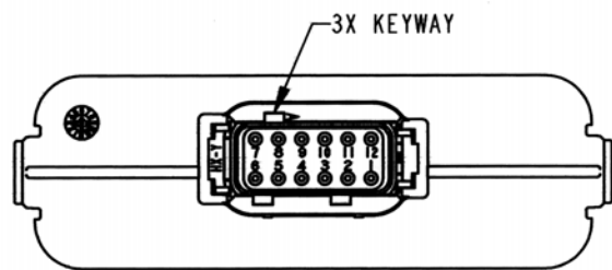
DTM13-12PA-R008 KEY -A- SLEEVE COLOR: GREY
