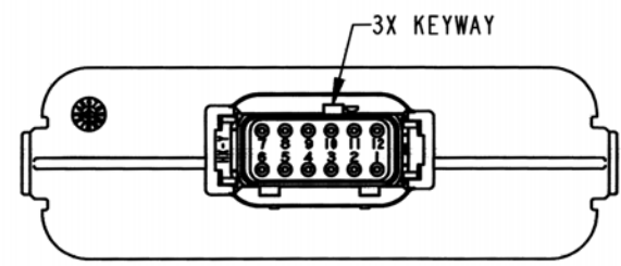
DTM13-12PD-R008 KEY -D- SLEEVE COLOR: BROWN
