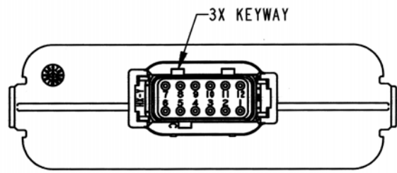
DTM13-12PC-R008 KEY -C- SLEEVE COLOR: GREEN
