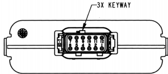
DTM13-12PB-R008 KEY -B- SLEEVE COLOR: BLACK
