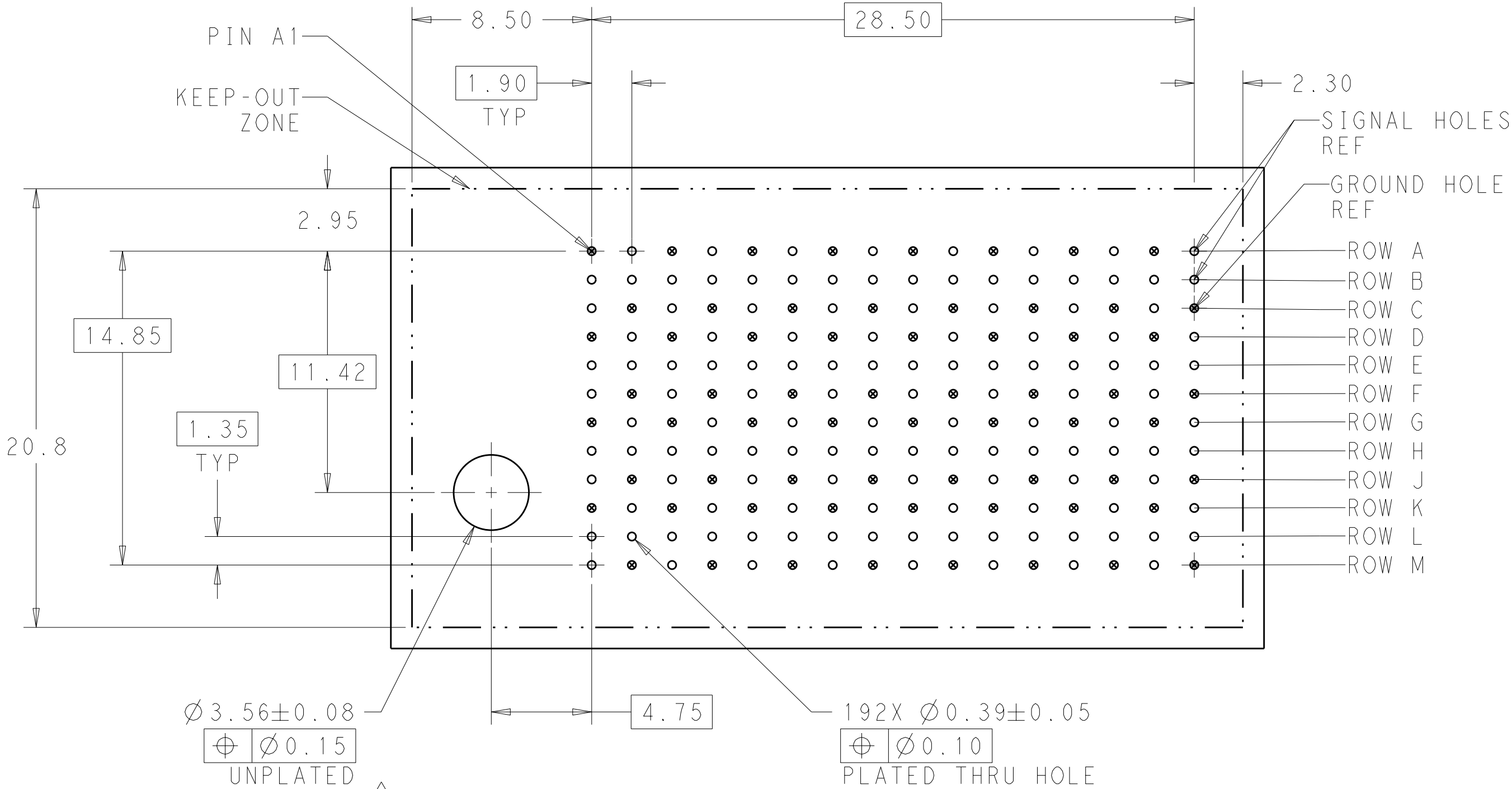
LEFT GUIDIED BACKPLANE HOLE PATTERN (CONNECTOR SIDE)
