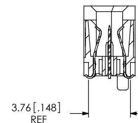
SECTION "G"-"G"
