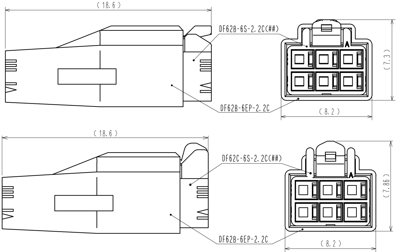
MATING FIGURE
