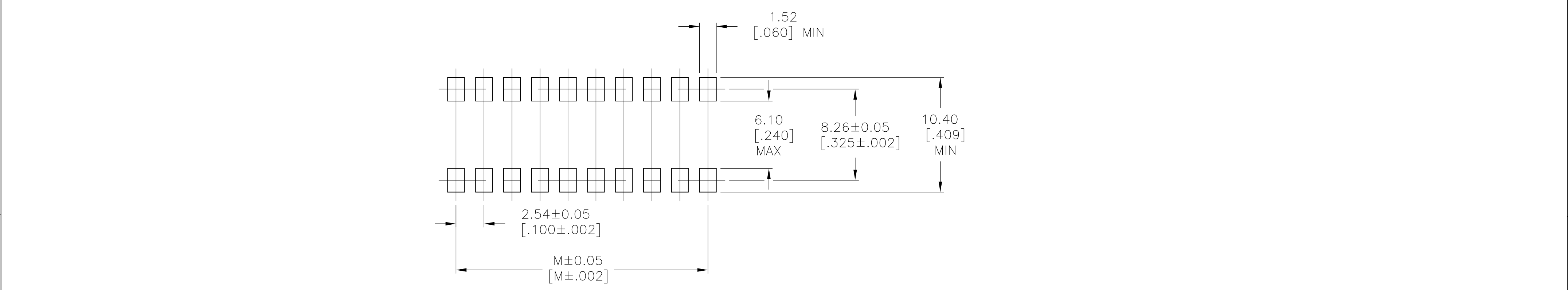
SURFACE MOUNT PAD LAYOUT
