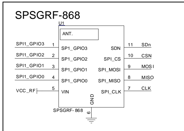
Figure 3: X-NUCLEO-IDS01A4 circuit schematic (3 of 3)
