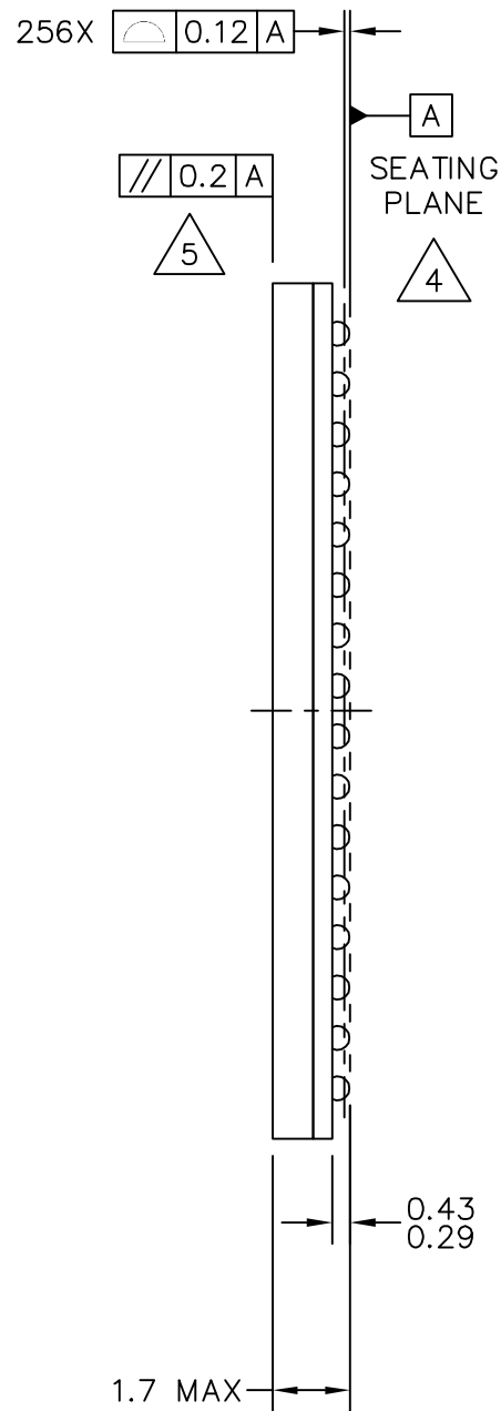
SIDE VIEW
