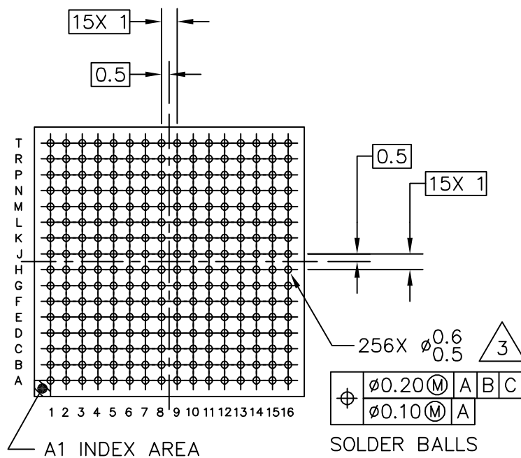
BOTTOM VIEW
