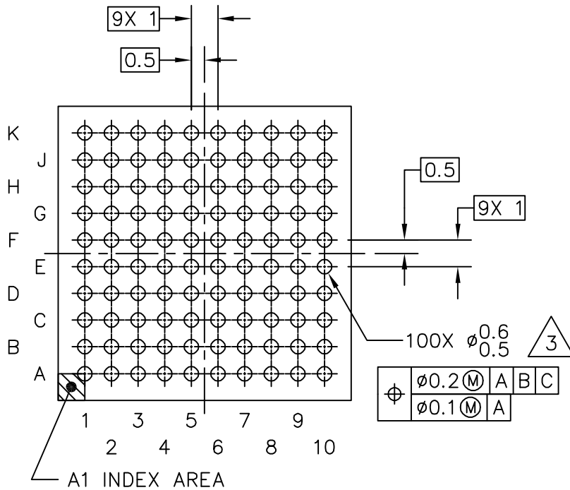
BOTTOM VIEW
