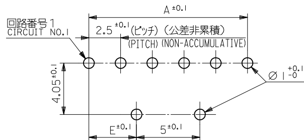
基板取付穴推奨寸法 (マウント面) (t=1.6) RECOMMENDED P.C. BOARD HOLE DIMENSION (MOUNTING SIDE) (SCALE 5:1)
