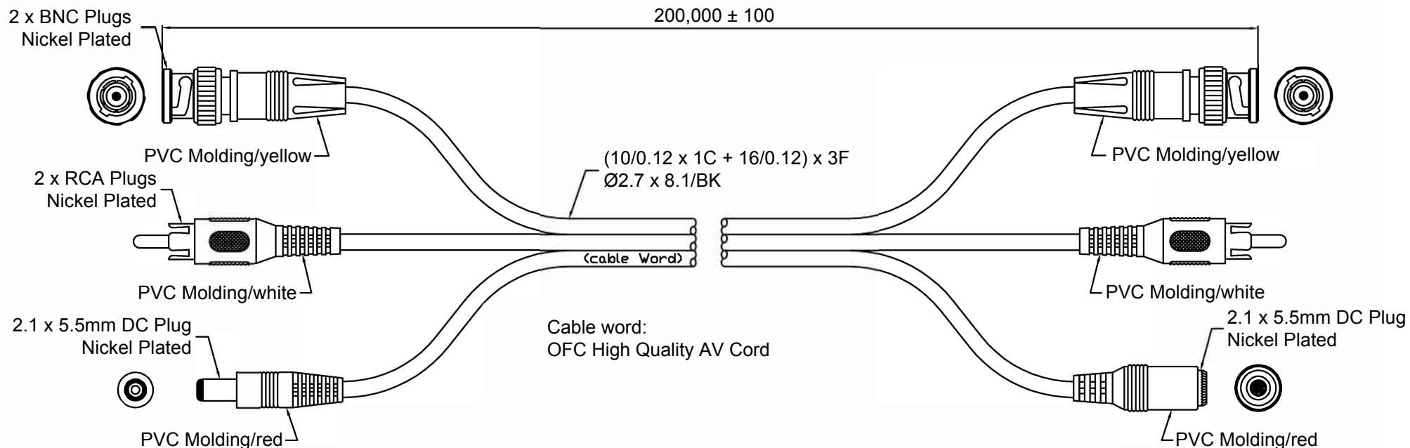
Soldered Drawing: 2.1 x 5.5mm DC Plug + RCA + BNC
