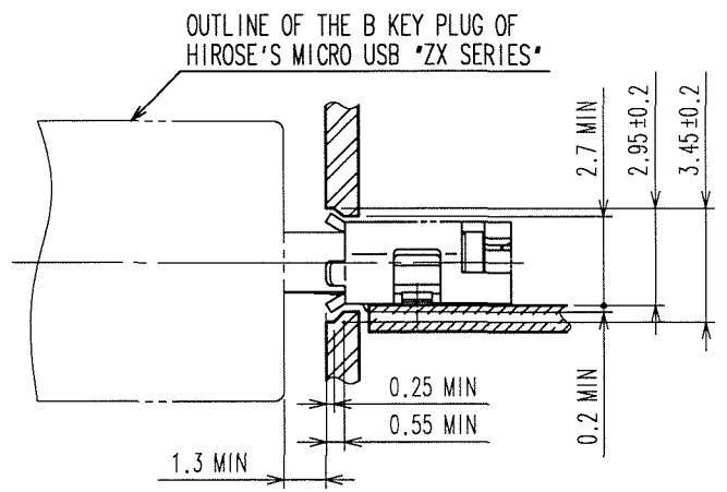
MATED WITH CORRESPONDING PLUG (4:1)
