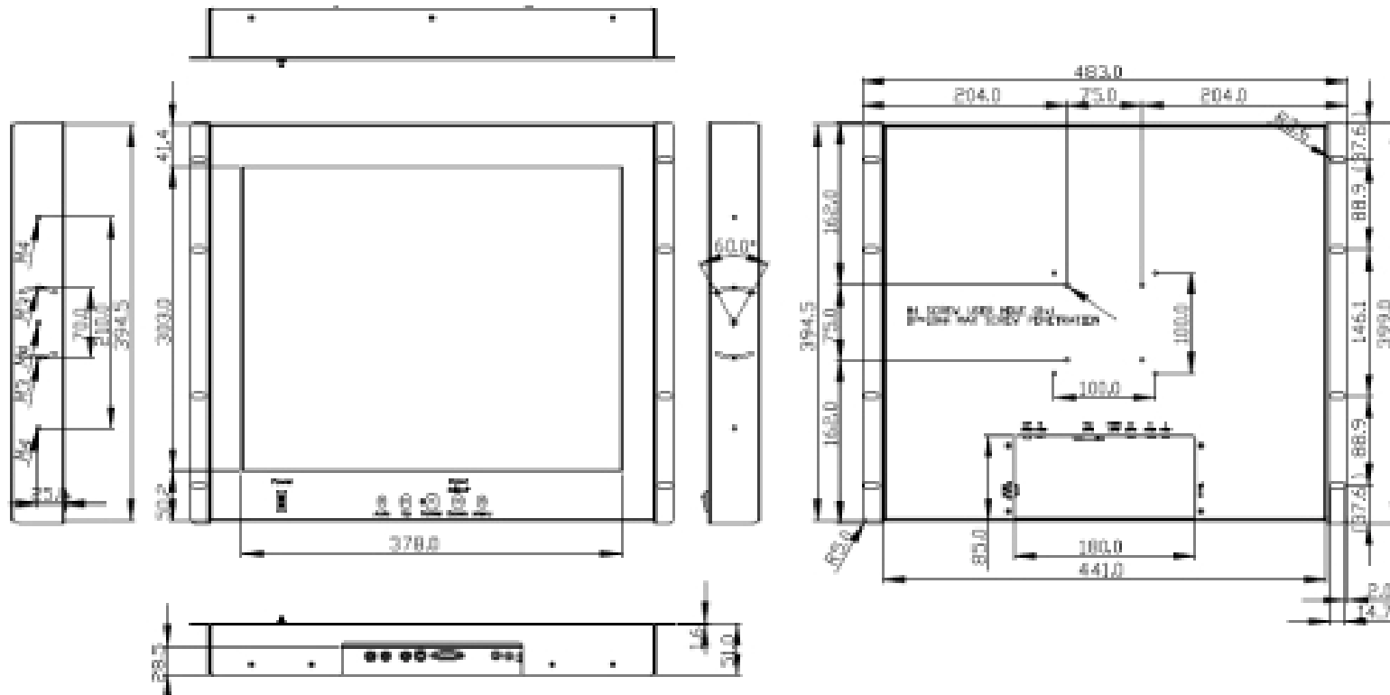
Line Drawing for: Model No. LRM1912 All sizes are in mm
