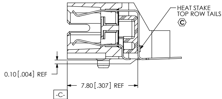
IN-PROCESS 11 (HEAT STAKE TOP ROW CONTACTS) (SEE INSPECTION VIEW 2 FOR ASSEMBLY ORIENTATION AND CPC'S)
