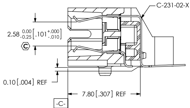
IN-PROCESS 10 (FILL TOP ROW) (SEE INSPECTION VIEW 2 FOR ASSEMBLY ORIENTATION AND CPC'S)
