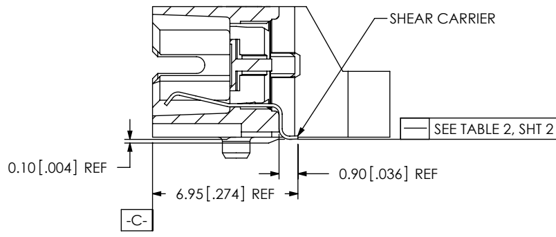
IN-PROCESS 5 (CUTOFF OF CARRIER) (SEE INSPECTION VIEW 1 FOR ASSEMBLY ORIENTATION AND CPC'S)
