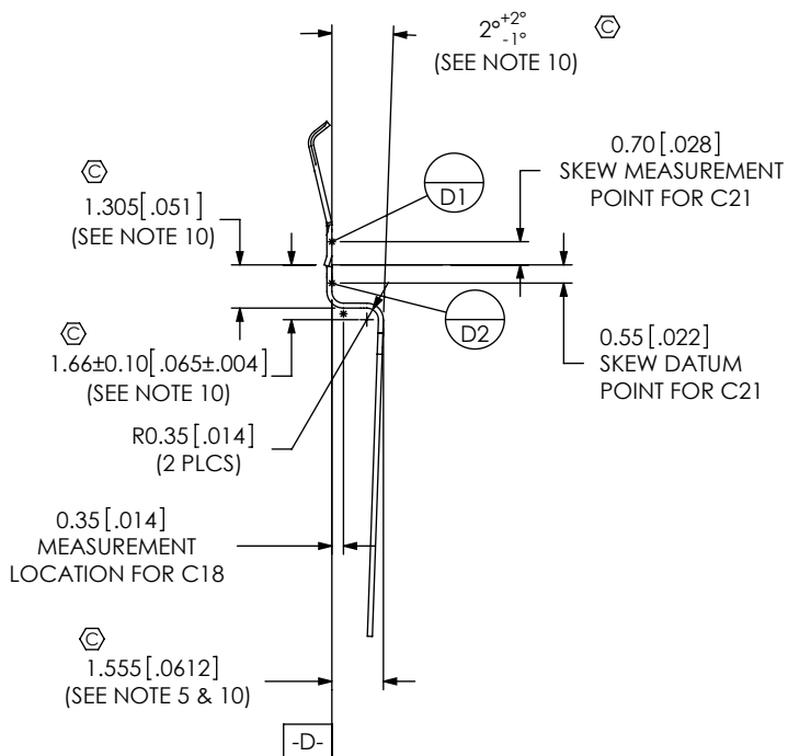
IN-PROCESS 3 (FORM 2 CONTACT C-231-03-X)
