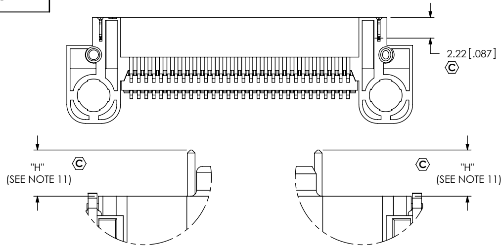
DETAIL 'G' SCALE 8:1
