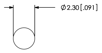
RECOMMENDED BOARD CUTOUT (M2 x 0.4)
