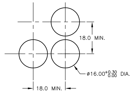
PANEL MOUNTING
