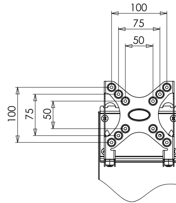
ALTERNATE VESA CONFIGURATION
