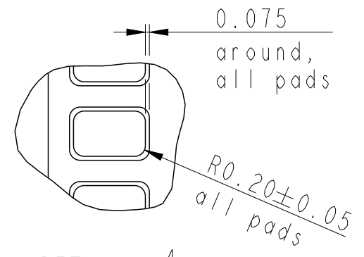
DETAIL 4 SCALE 10:1
