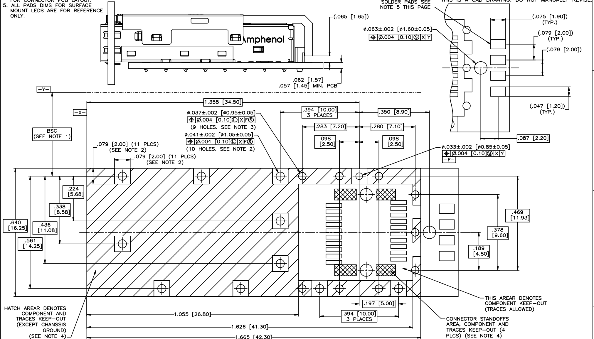
RECOMMENDED SFP HOST BOARD LAYOUT (ONE SIDE CAGE MOUNTING) (SCALE 4:1)
