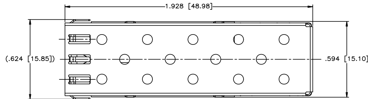
TOP VIEW (CAGE SHOWN ONLY)
