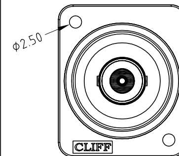
CP303090X - Ø2.50 PLAIN HOLES
