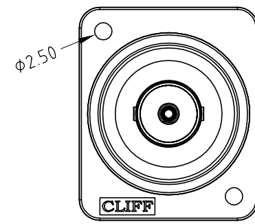
CP303095X - Ø2.50 PLAIN HOLES
