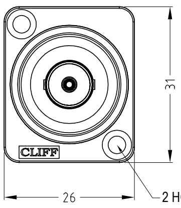
CP303095 - CSK HOLES
