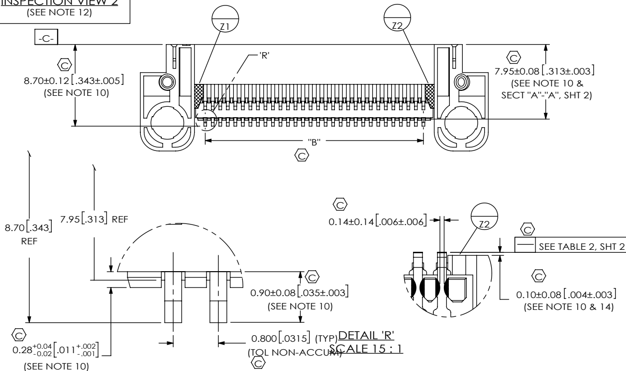
IN-PROCESS 12 (CUTOFF OF CARRIER) (SEE INSPECTION VIEW 2 FOR ASSEMBLY ORIENTATION AND CPC'S)
