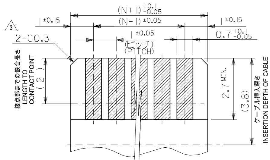
適合FPC/FFC推奨寸法 APPLICABLE FPC/FFC RECOMMENDED DIMENSION (仕上り厚さ: 0.3 ±0.05) (THICKNESS: 0.3 ±0.05)
