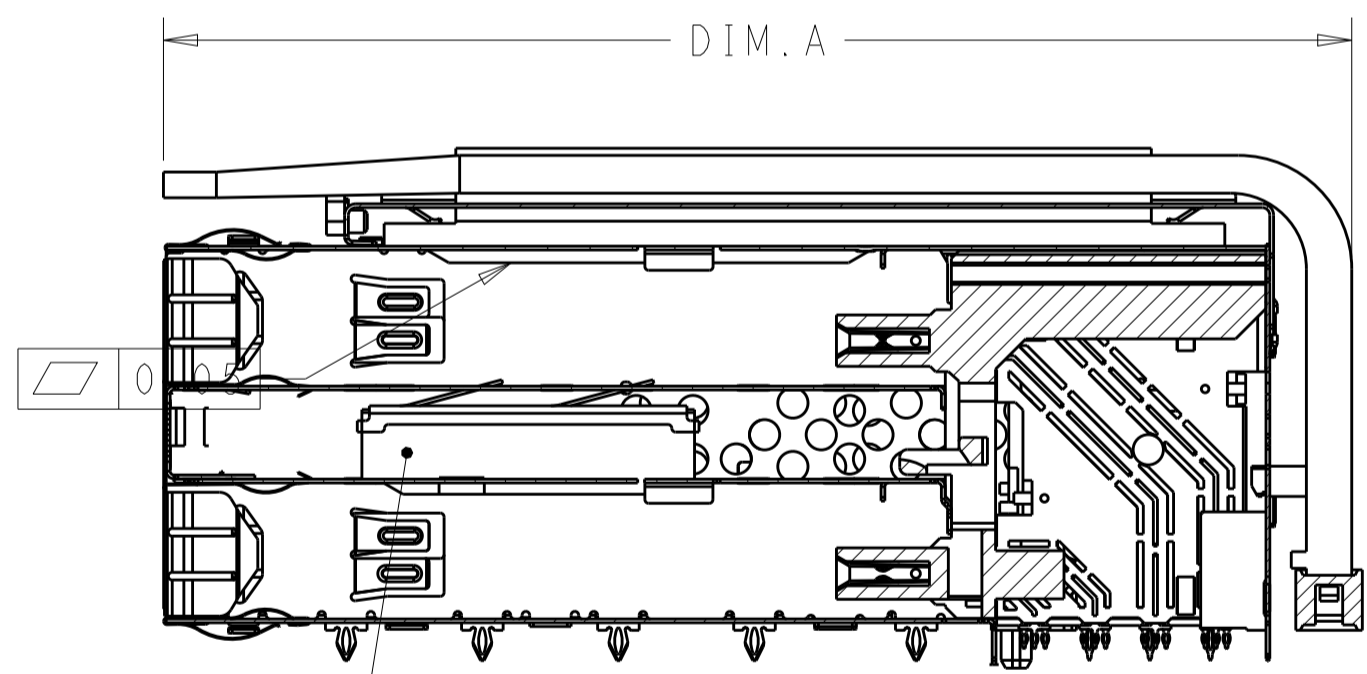
2299924-1 1-2299924-1 SECTION VIEW SECTION V-V SCALE 2:1
