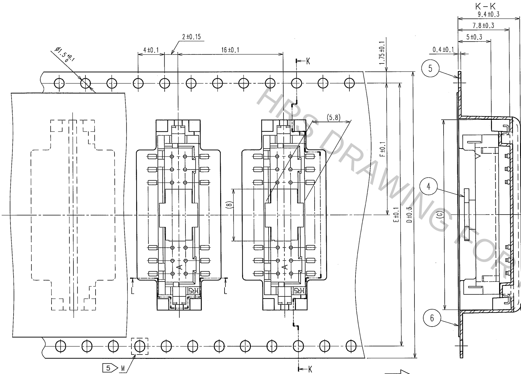
STYLE AND DIMENSION OF REEL
