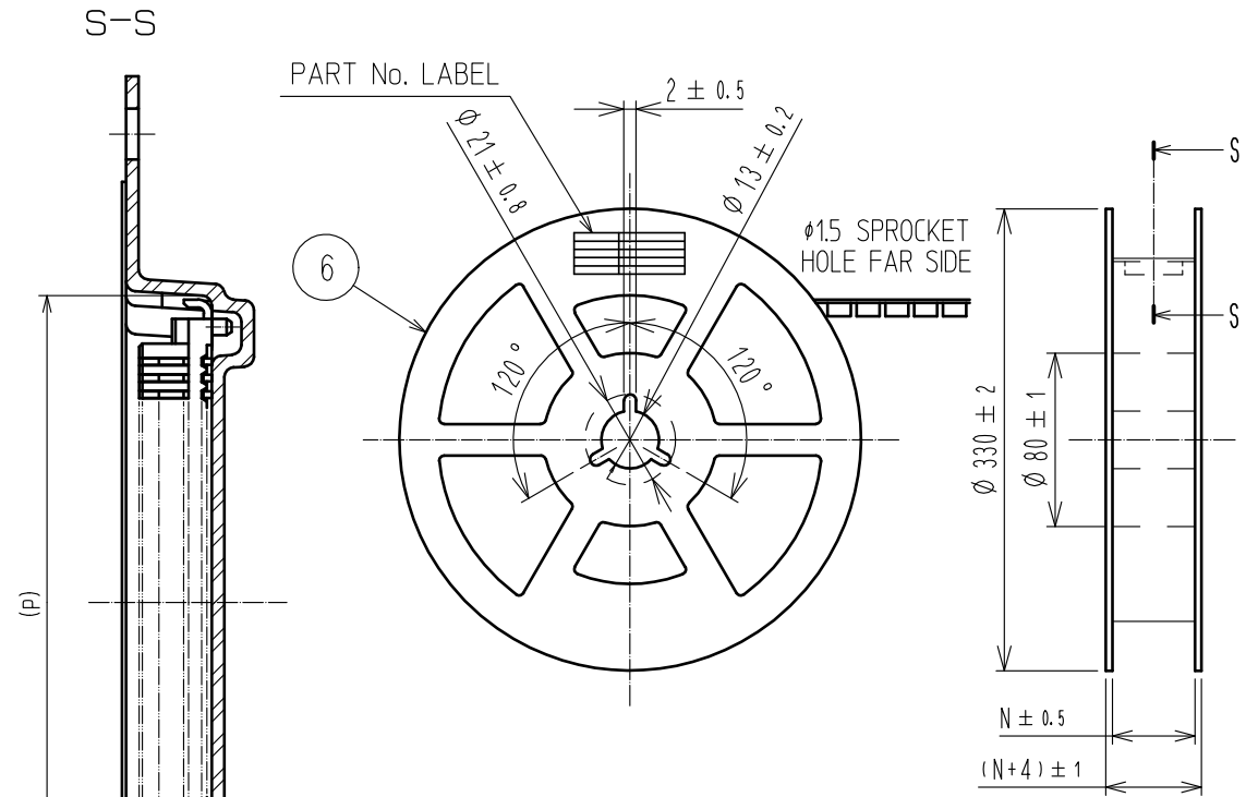
△ STYLE AND DIMENTION OF REEL (FREE)
