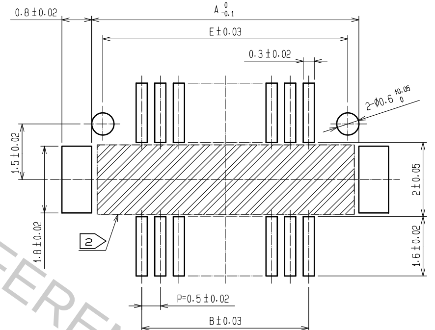
RECOMMENDED PATTERN(10:1)
