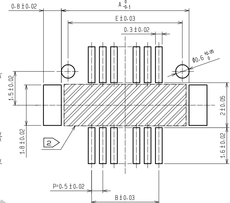
RECOMMENDED PATTERN (10:1)
