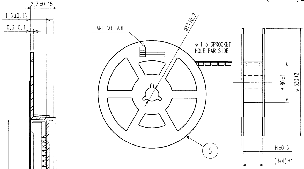
STYLE AND DIMENSION OF REEL (FREE)△
