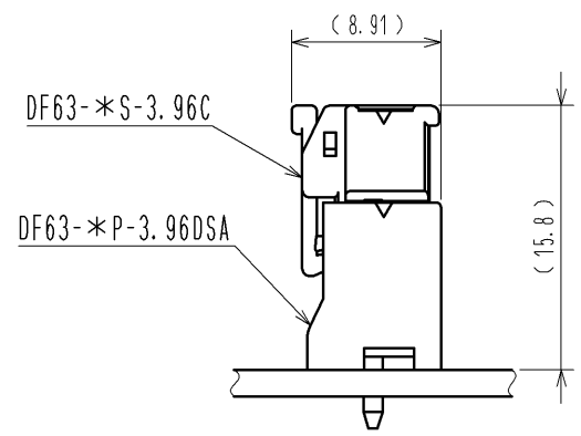
Mating Figure
