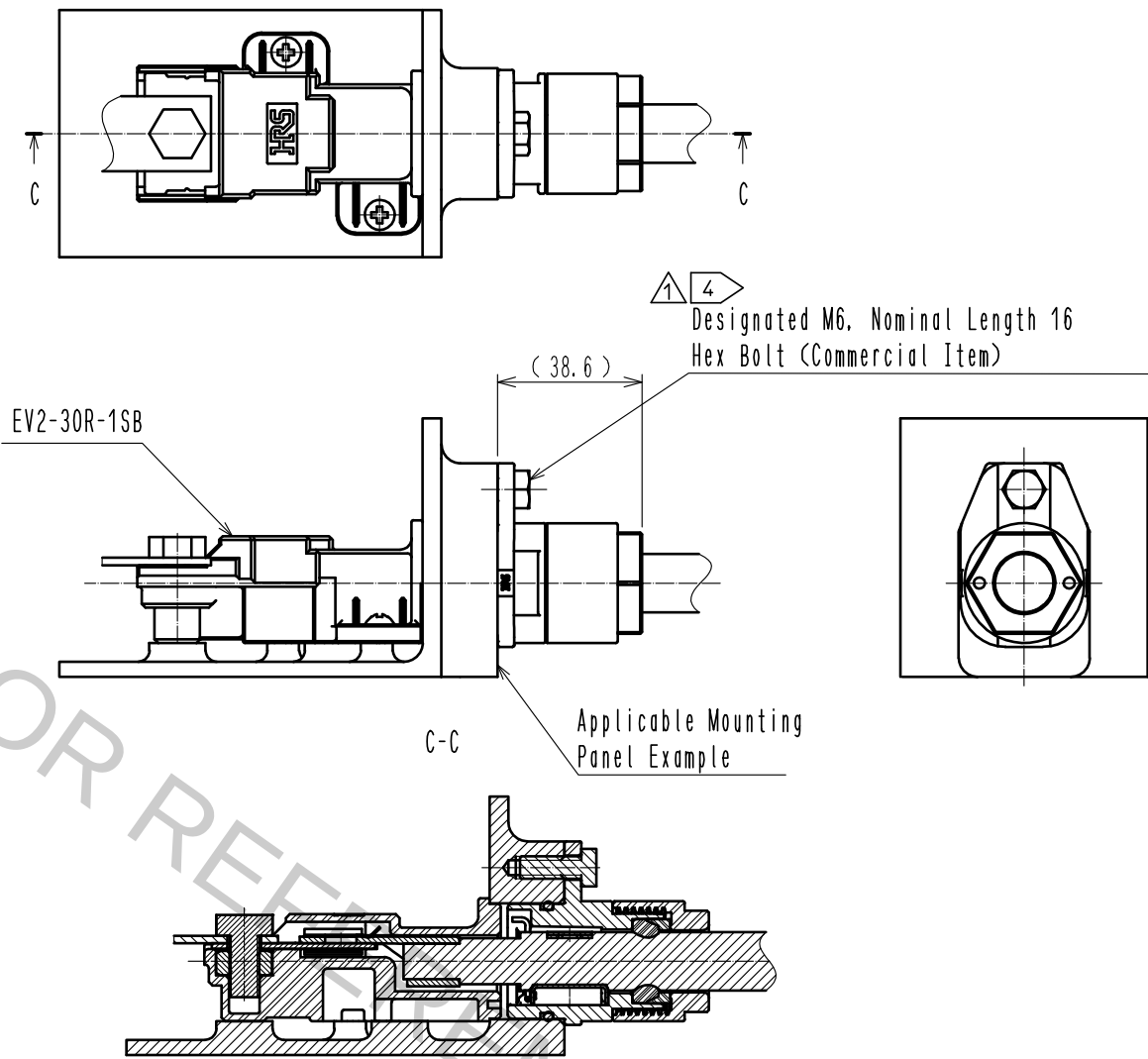
6/8 Mated Condition Diagram(1:2)
