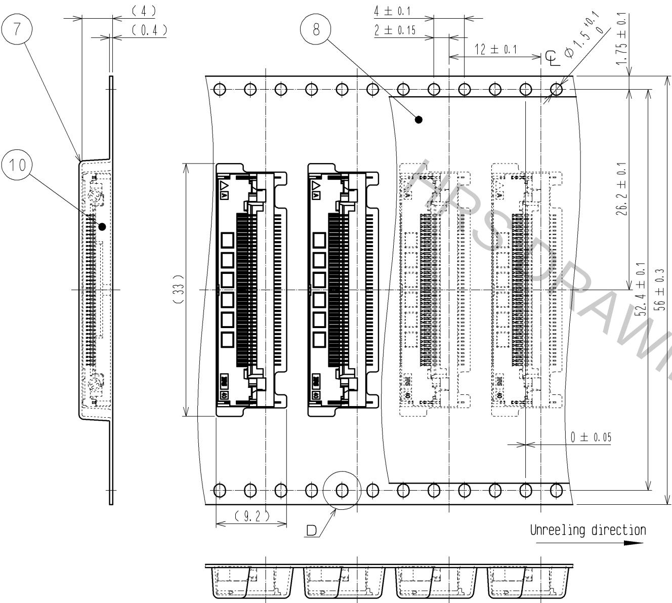
Embossed carrier tape dimensions (2:1)
