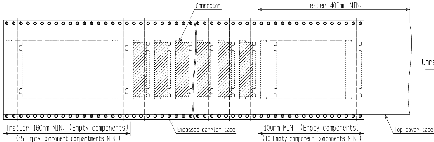
Leader ,trailer dimensions (SCALE:FREE)
