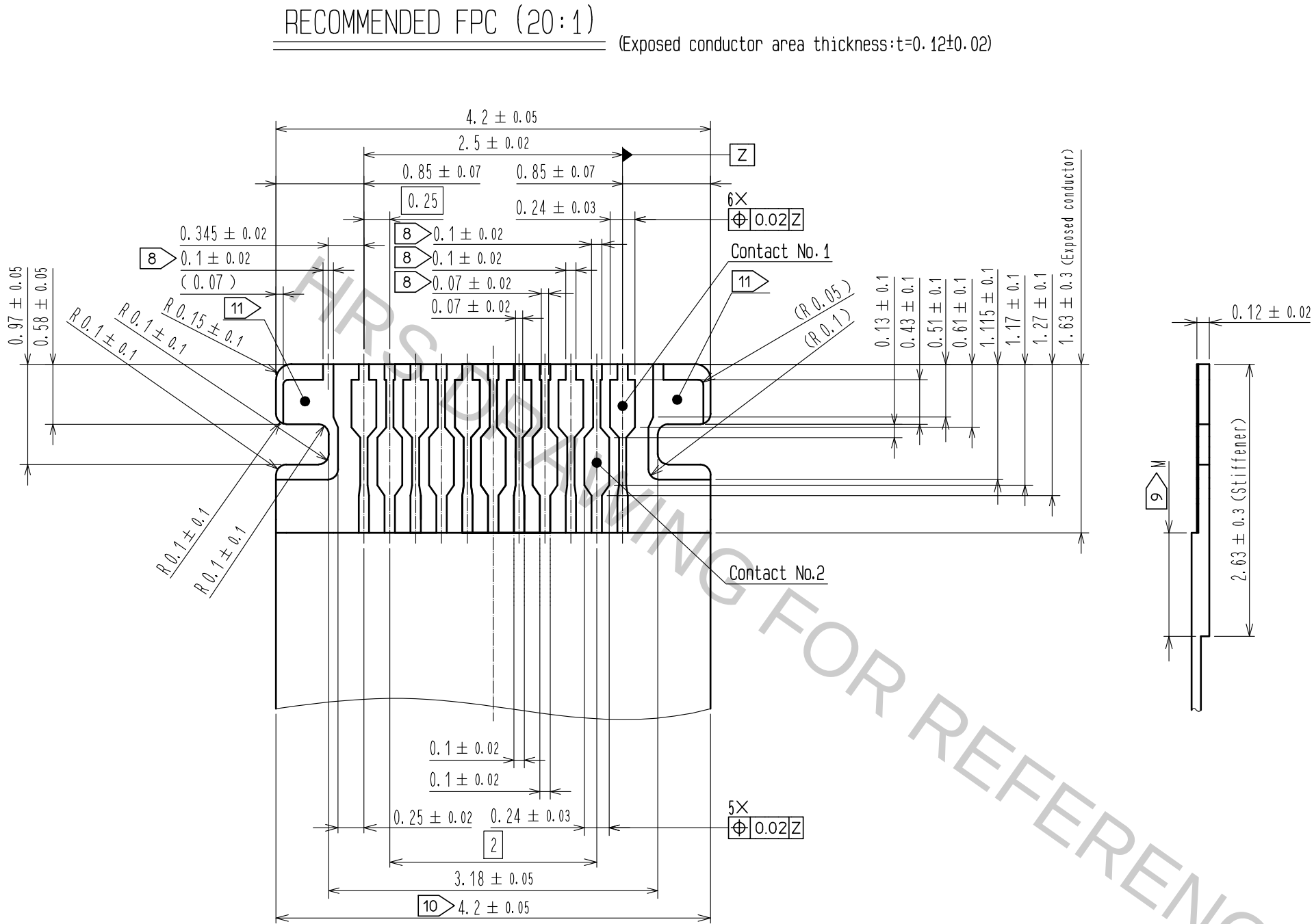
FPC CONFIGURATION (REFERENCE EXAMPLE) (FREE)
