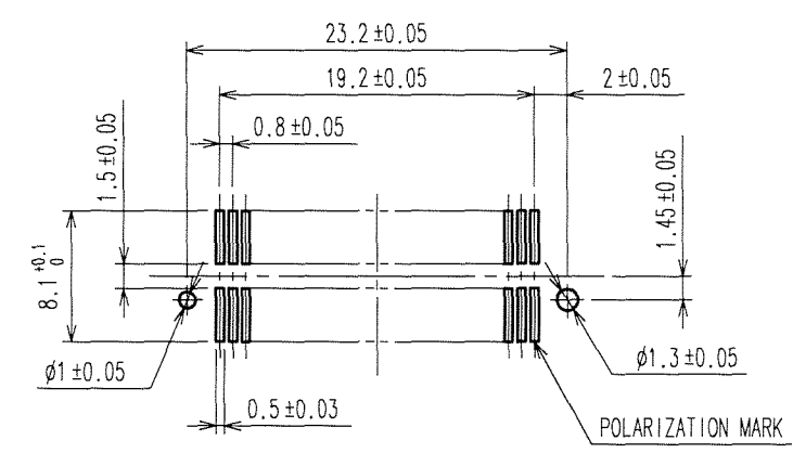
RECOMMENDED LAND PATTERN DIMENSION OF PCB (MOUNTING SIDE)
