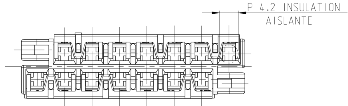
DETALLE CAJA CON BISAGRA CERRADA HOUSING WITH CLOSED FLAP
