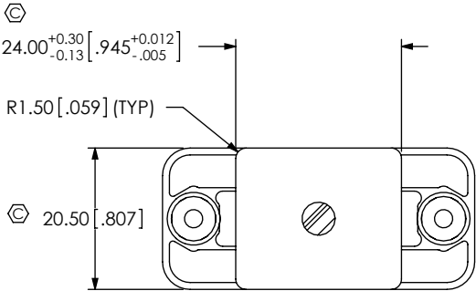
SECTION "H"-"H"
