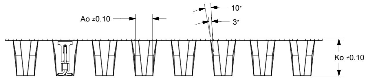
PART PACK IN E/TAPE ORIENTATION(FOR REF USE)
