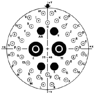
Contact Layout
