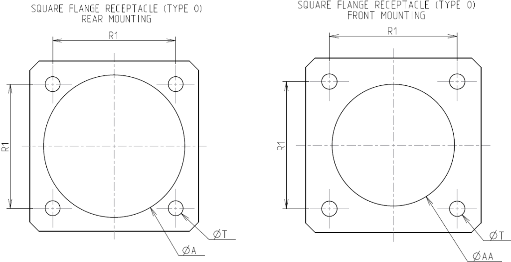
Panel Cutout
