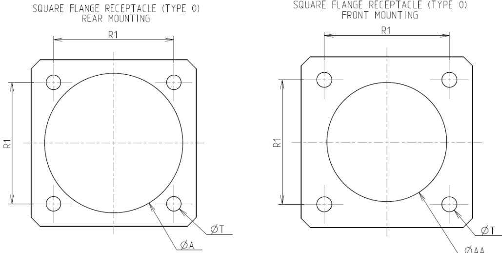
Panel Cutout
