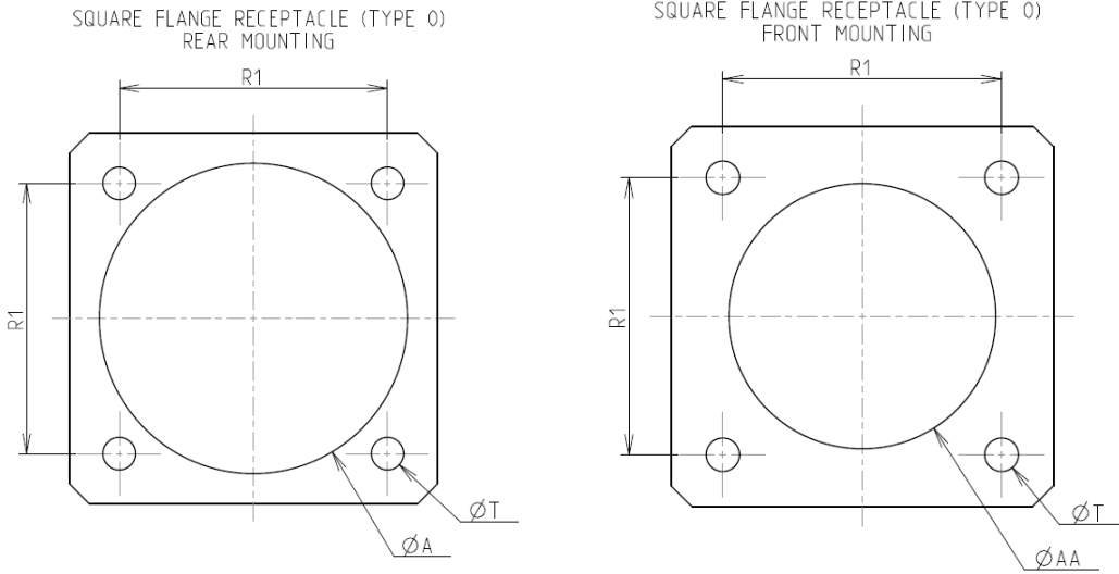
Panel Cutout
