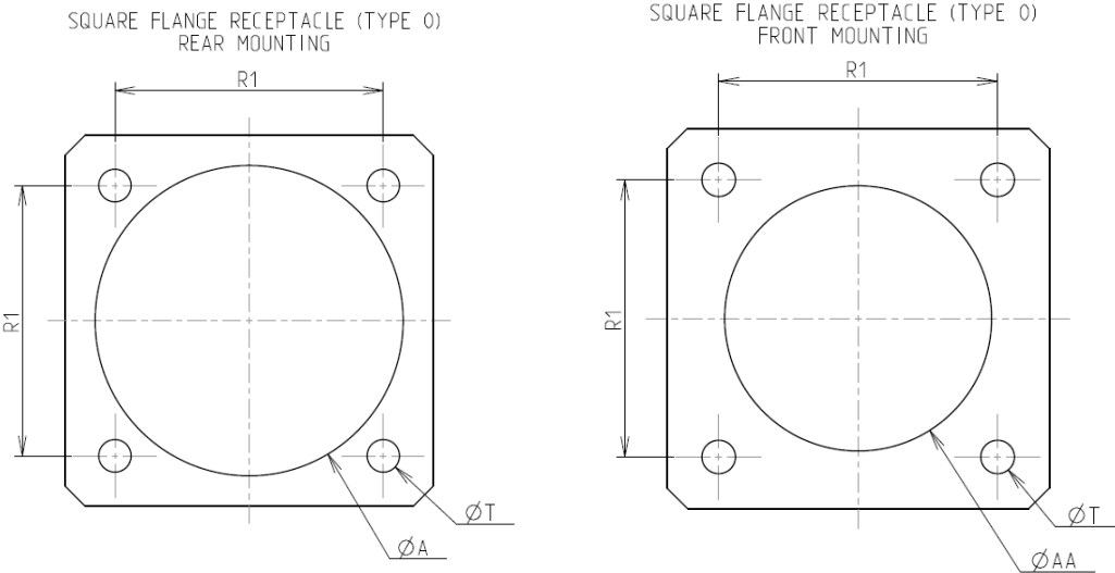
Panel Cutout
