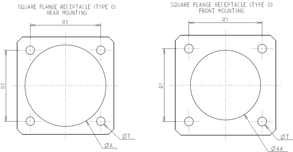
Panel Cutout
