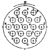
Contact Layout
