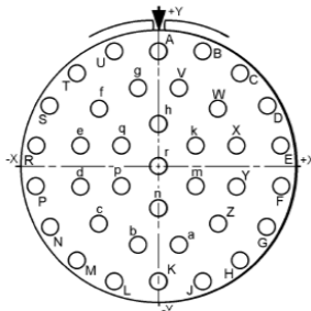
Contact Layout
