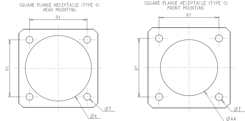
Panel Cutout
