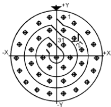
Contact Layout
