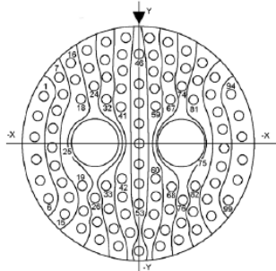
Contact Layout
