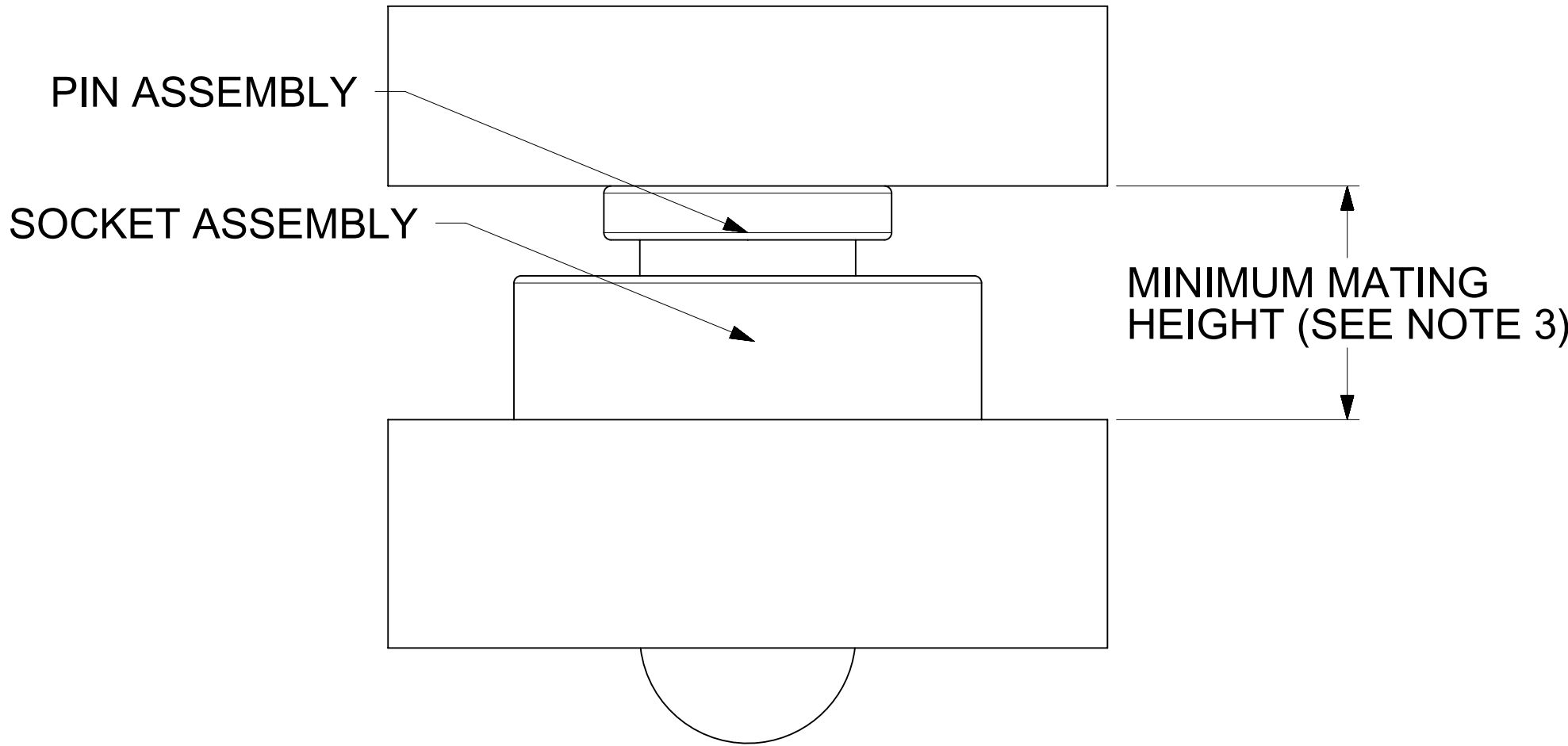
MATING PROFILE
